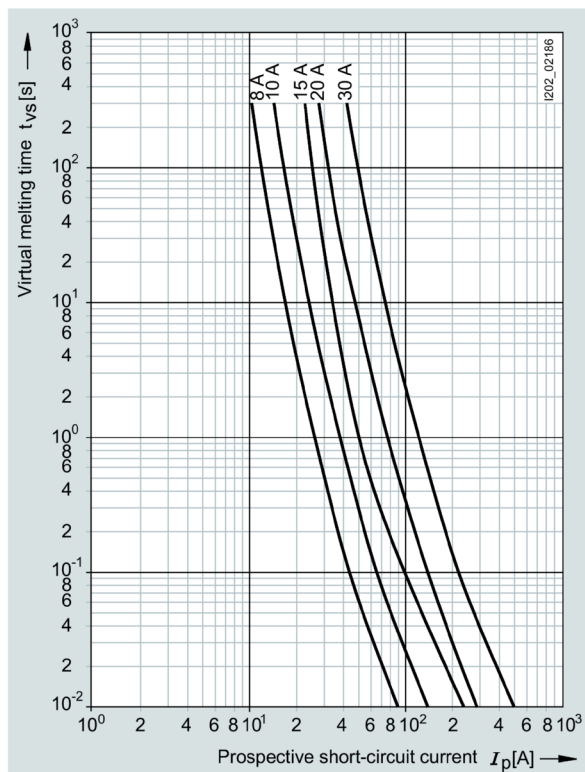
Time/current characteristic curves diagram
