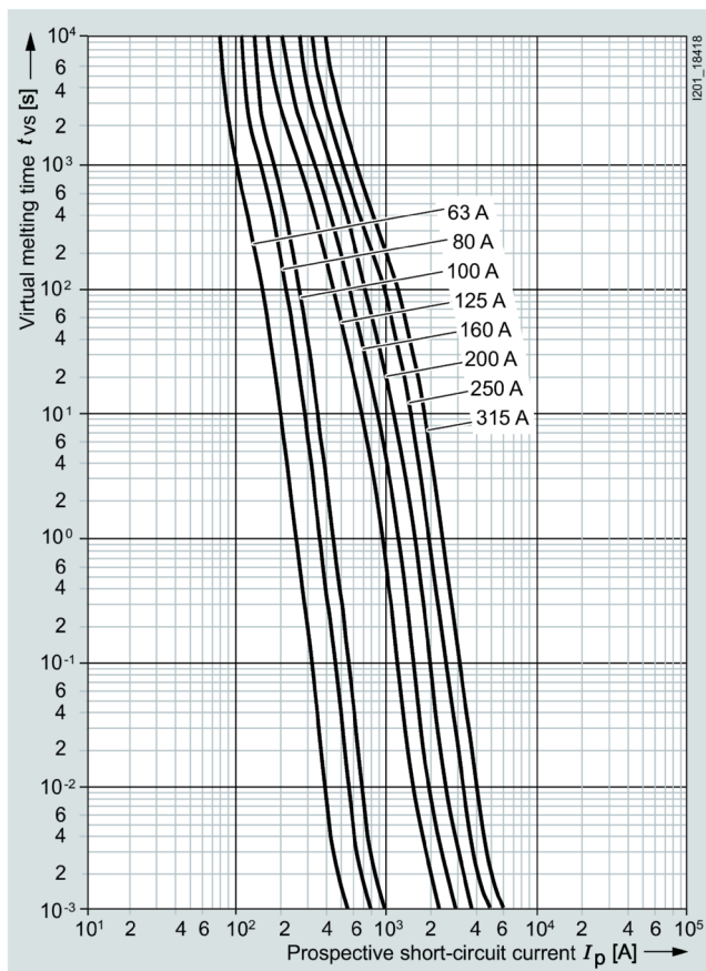
Time/current characteristic curves diagram 1500 V
