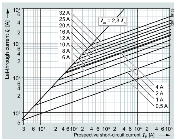
Current limiting diagram
