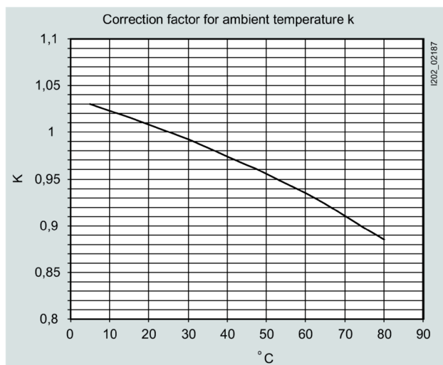
Characteristic curves diagram, correction factor for ambient temperature
