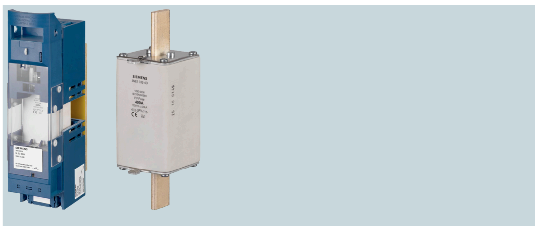
Figure 8-2 PV LV HRC fuse system, 3NH73..-4, 3NE13..-4D
