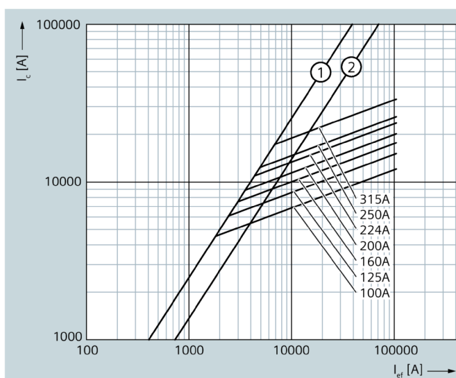
Current limiting diagram, operational class gG
