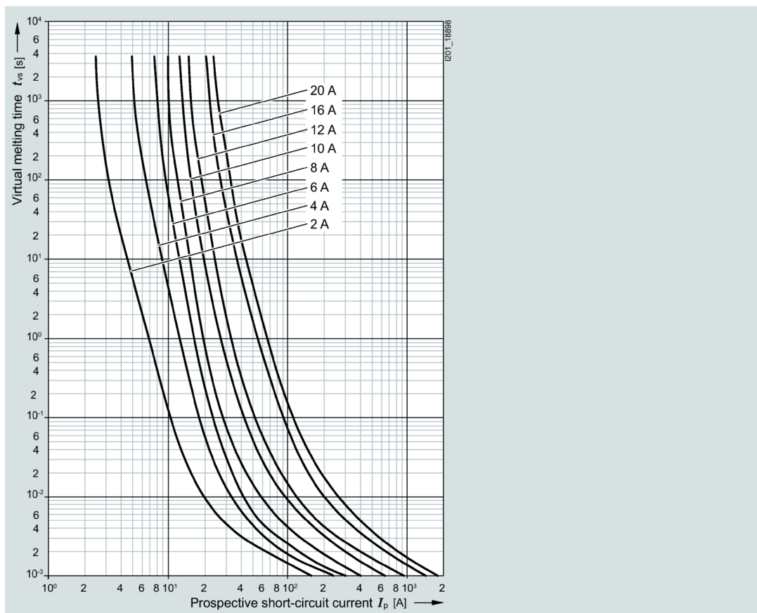
Time/current characteristic curves diagram 3NW600.-4
