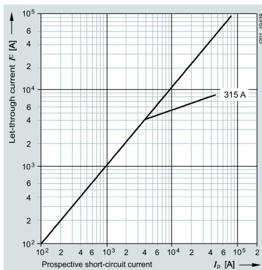
Let-through characteristic curves (current limiting at 50 Hz)
