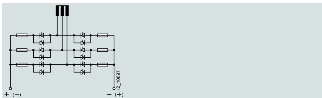
Six-pulse bridge circuit B6 with branch fuses (reversible connection)
