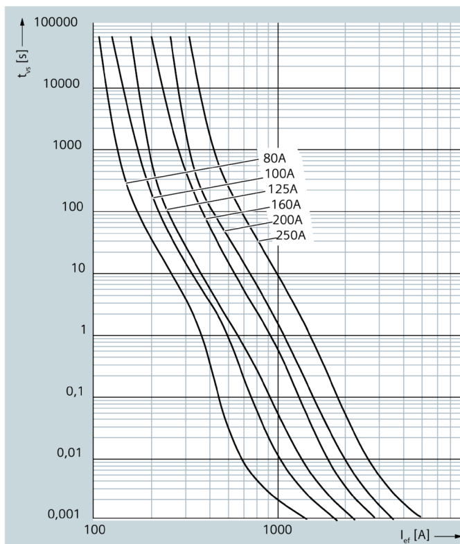
Time/current characteristic curves diagram, operational class gFF
