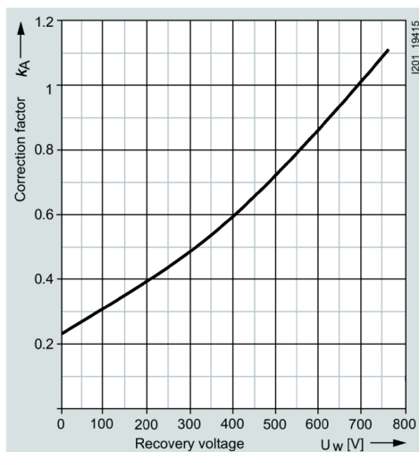
Correction factor k_A for breaking I^2t value
