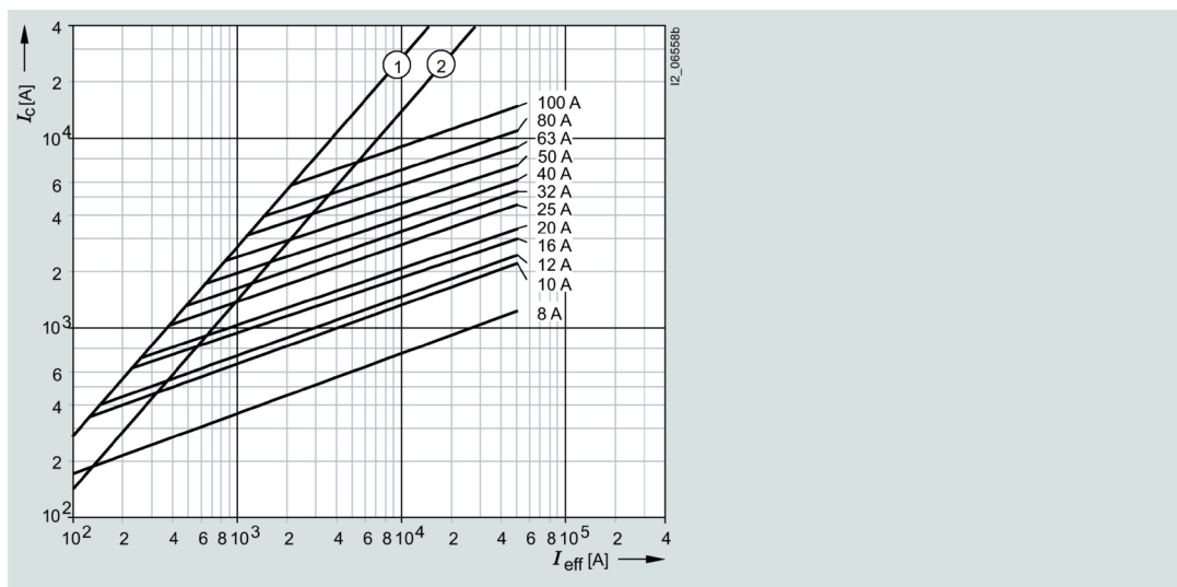
Current limiting diagram
