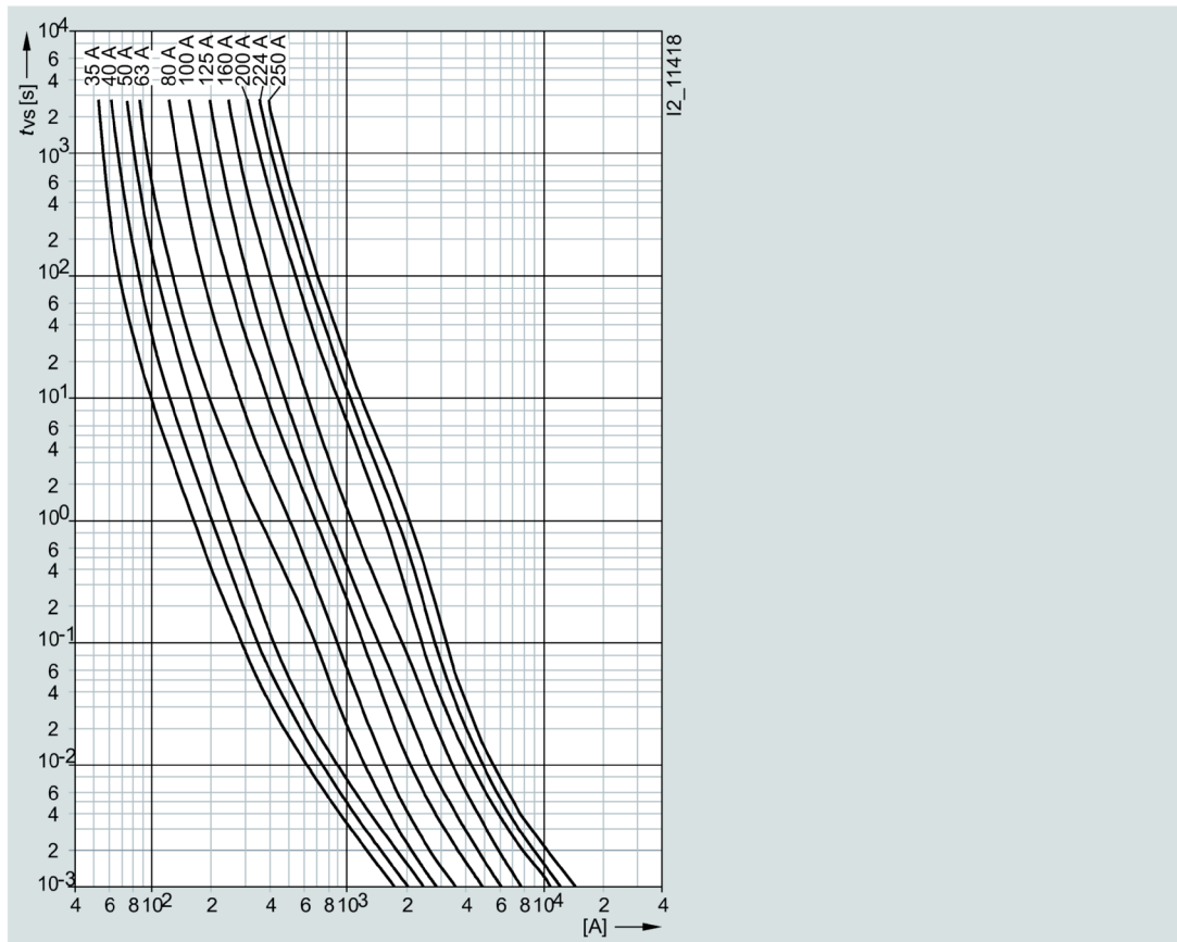
Time/current characteristic curves diagram
