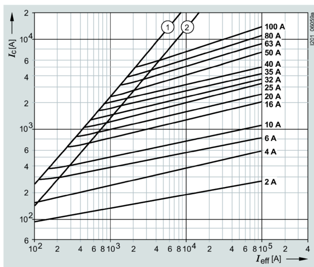
Current limiting diagram
