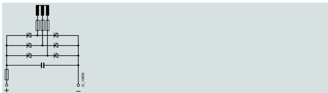
Six-pulse bridge circuit B6 with branch fuses
