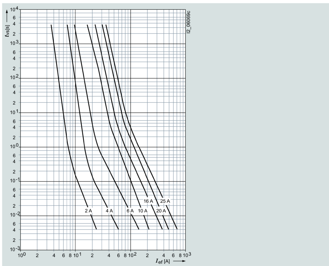
Time/current characteristic curves diagram
